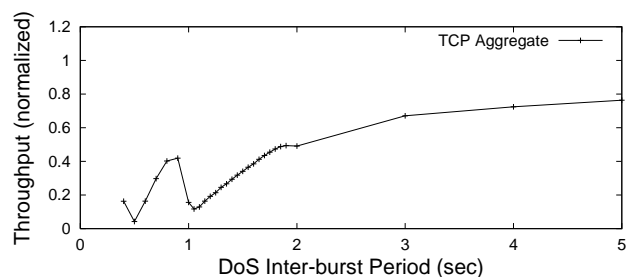
Figure 6: DoS and aggregated TCP flows
