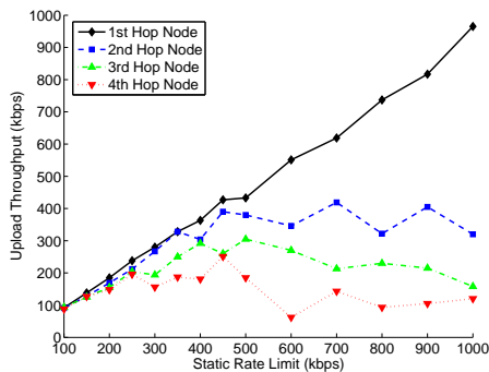
Figure 14: The fully backlogged parking lot traffic matrix upstream with each flow equally rate limited at the source.
