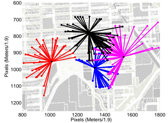
Figure 8: Backhaul link measurements from four fixed locations.
