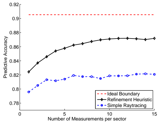
Figure 9: Accuracy of boundary refinement algorithm for the coverage region of mesh nodes in GoogleWiFi.
