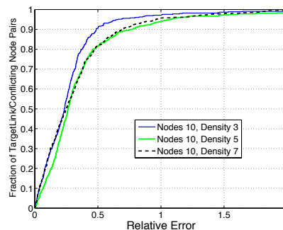
Figure 14: Throughput prediction sensitivity to density (900 kbps).
