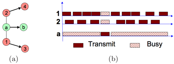
Figure 1: Example of transmission alignment due to (lack of) carrier sensing.
