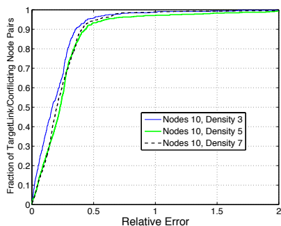
Figure 12: Throughput prediction sensitivity to density (600 kbps).
