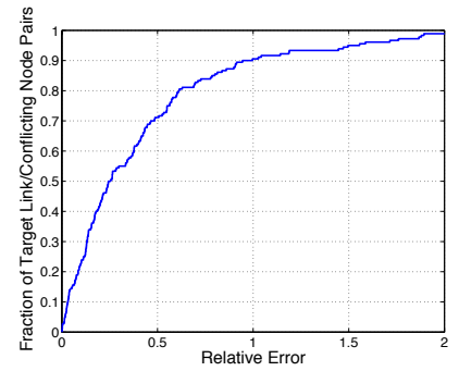
Figure 5: Throughput increase estimation (testbed).
