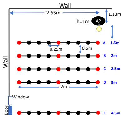
Figure 6: Testbed setup for dual-band experiments.
